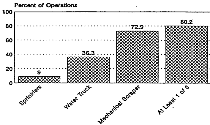
Figure 1: Dust control practices on beef feedlots of 1,000 or more head.
