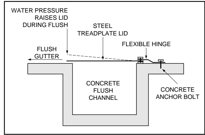
Figure 8. Cross-section of raising-lid flush channel.
