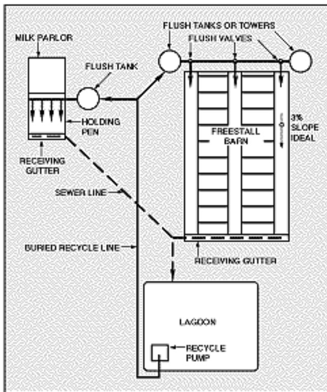
Figure 1. Schematic of typical components in a dairy flush system.
